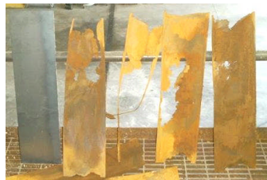
Figure 1a: 190 L/m Sacrificial Metal Blades (New and Used)
